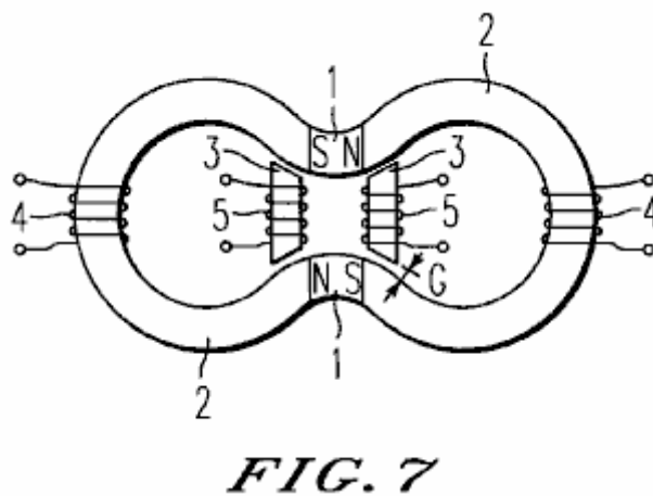
Fig.7 is a third embodiment of the static magnet dynamo involved in this invention.
