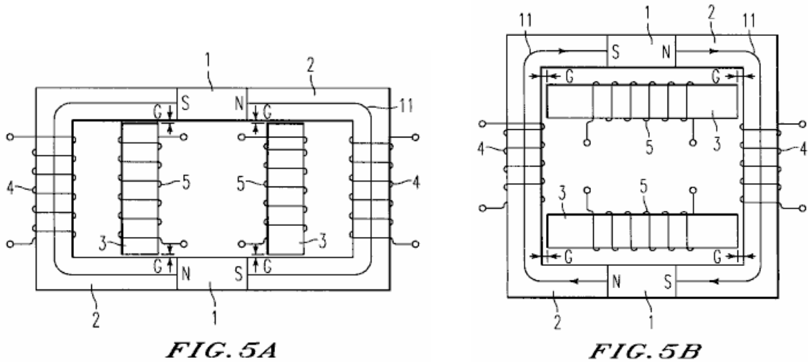
Fig.5 is a first embodiment of the static magnet dynamo involved in this invention.
