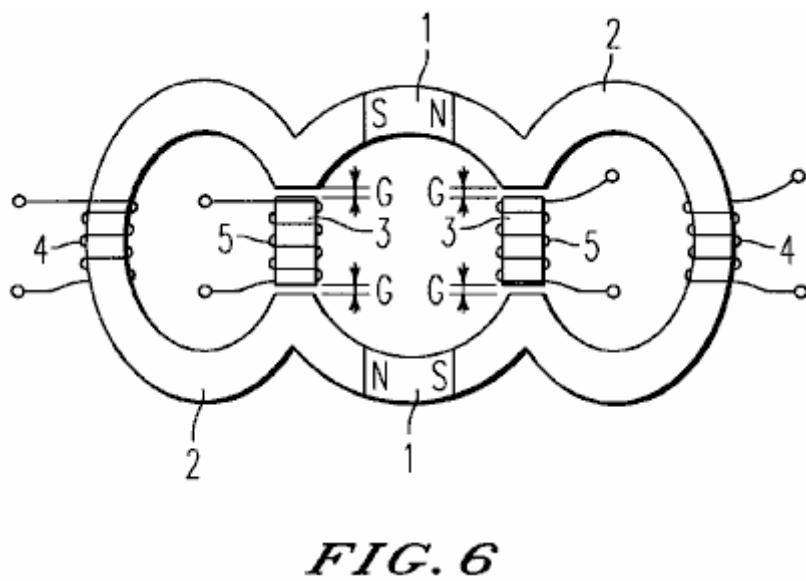
Fig.6 is a second embodiment of the static magnet dynamo involved in this invention.
